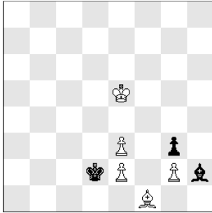
h#6 (5+3)
