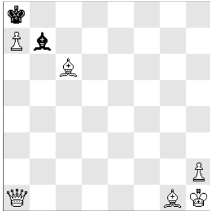
s#7* (6+2)
