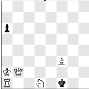
s#7 (5+2)
